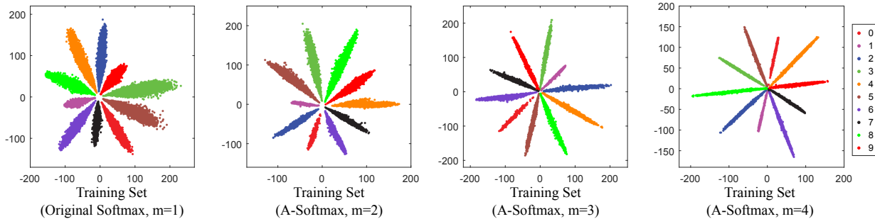
Figure 12: 2-D MNIST visualization of features learned by the softmax loss and the A-Softmax loss ( m = 2, 3, 4 ).
