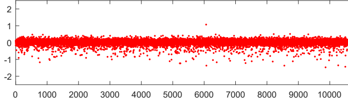
Figure 10: Biases of last fully connected layer learned in CASIA-WebFace dataset.
